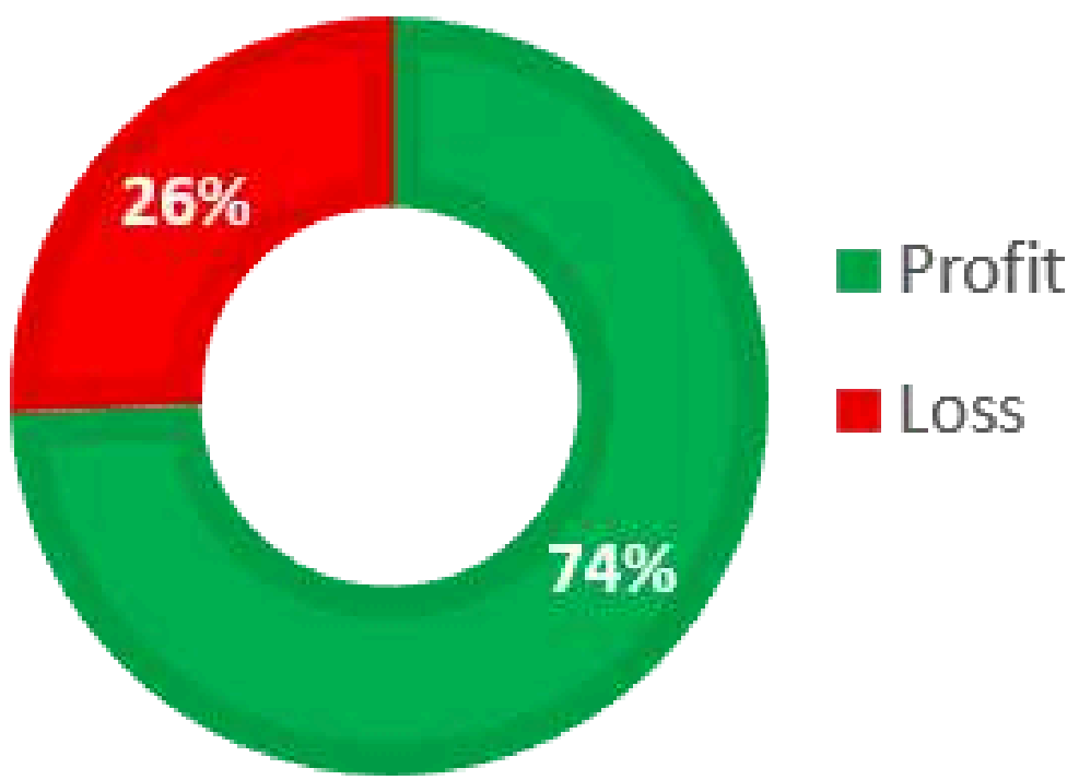
WIN RATE
