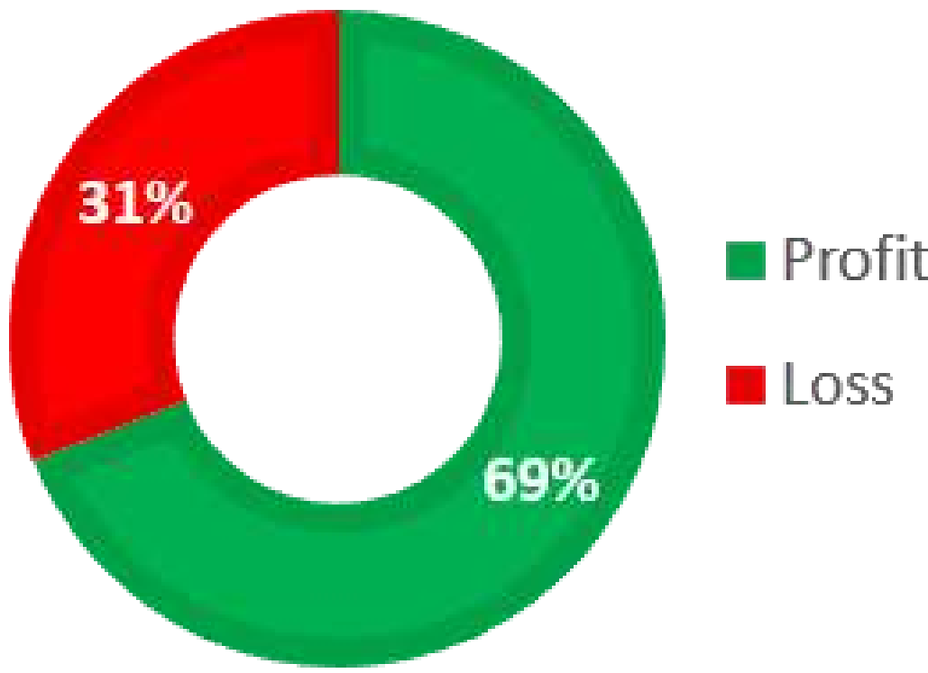
WIN RATE
