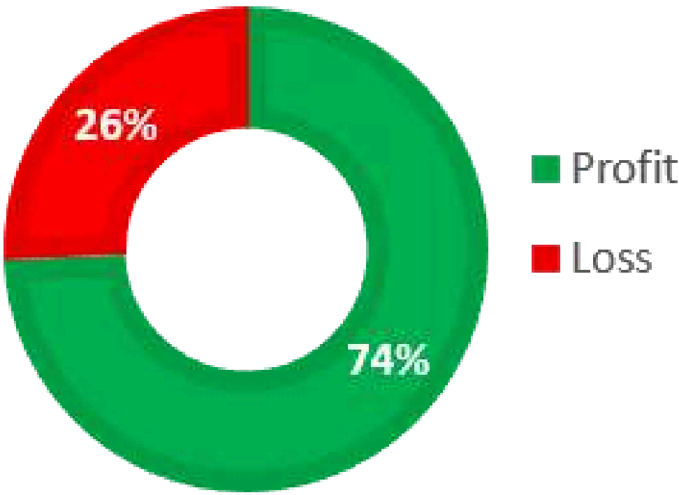
WIN RATE
