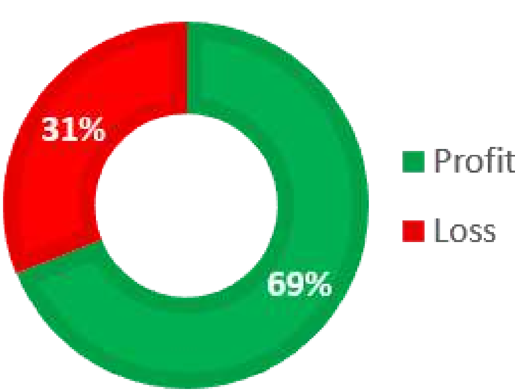
WIN RATE
