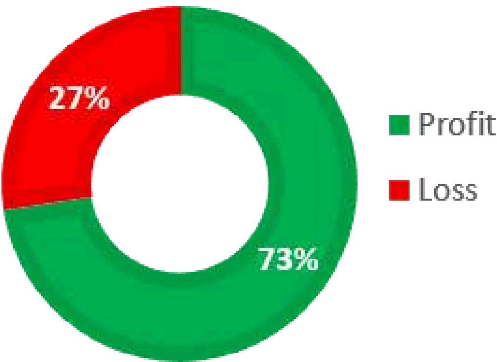
WIN RATE
